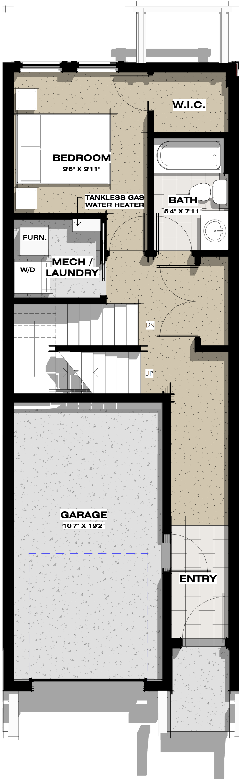
MAIN FLOOR PLAN 1/4" = 1'-0" MAIN FLOOR LIVING SPACE 417 sq.ft. GARAGE 208 sq.ft.
