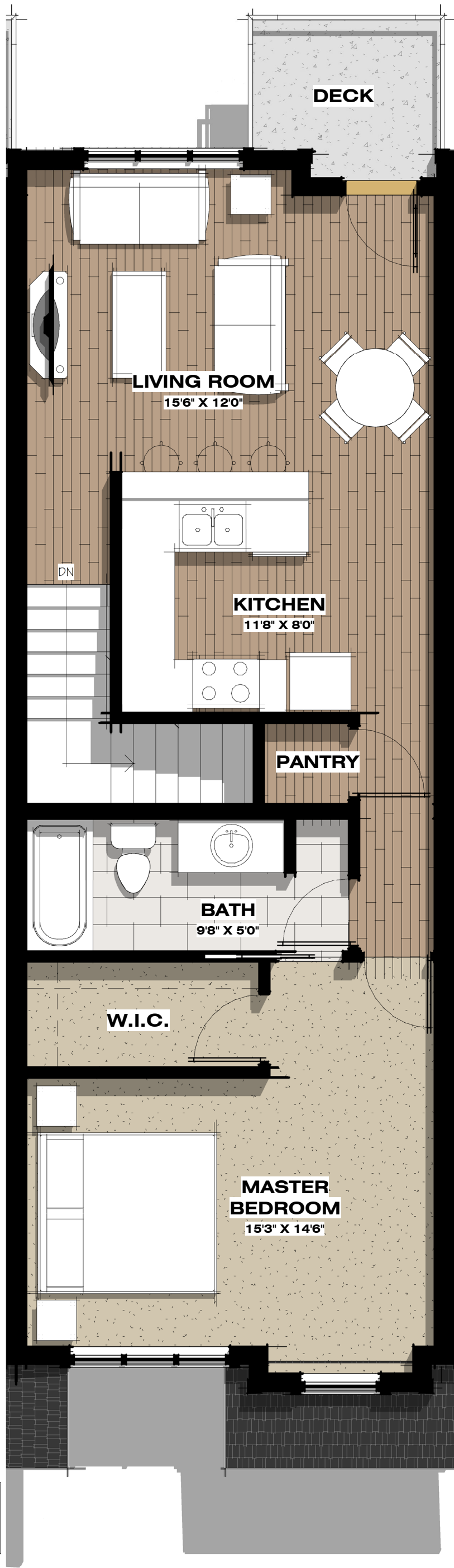
SECOND FLOOR PLAN 1/4" = 1'-0" SECOND FLOOR LIVING SPACE 665 sq.ft.
